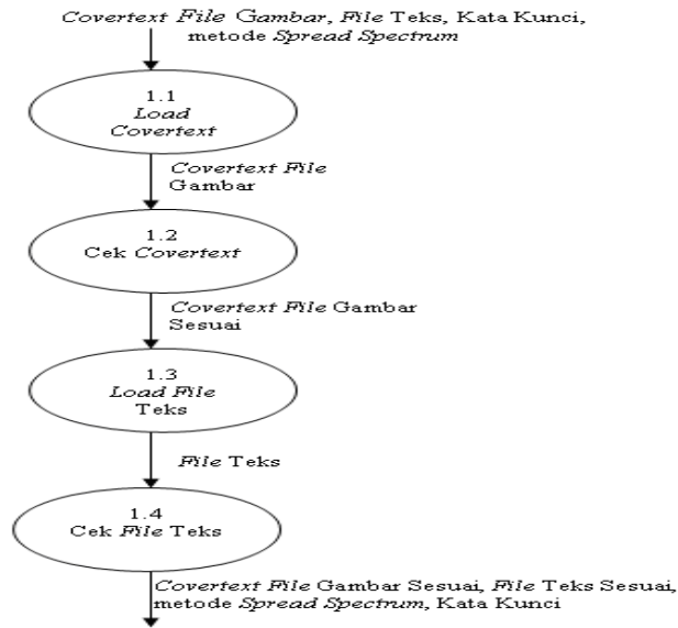
Gambar 5 DFD Level Dua Proses Cek Data Metode Spread Spectrum
